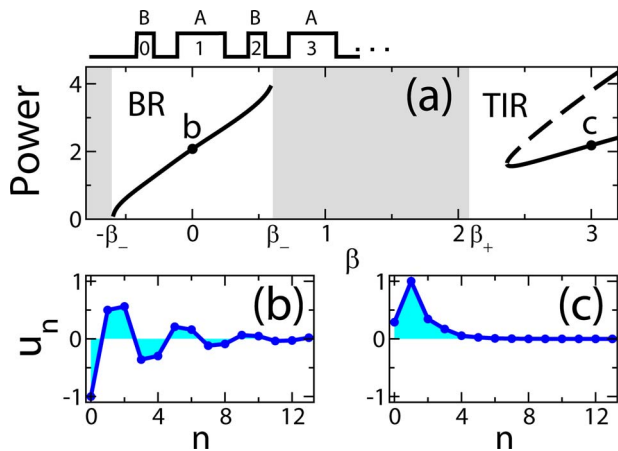
Fig. 3. (Color online) (a) Families of nonlinear Tamm (gap) states and discrete surface solitons in the binary array truncated at the narrow waveguide. The solid and dashed curves correspond to the stable and unstable branches, respectively. A schematic of the array is shown at the top. (b), (c) Characteristic examples of the soliton profiles corresponding to points b and c in (a). The detuning parameter of the array is \rho=0.6 .
