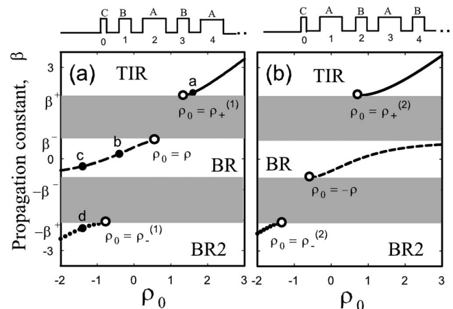
Fig. 1. (a), (b) Spectra of the linear surface modes in a binary array of alternating thick (A) and thin (B) optical waveguides with a surface defect (C) for two configurations of a semi-infinite structure shown schematically at the top. The shaded areas mark two bands of an infinite binary array ( \rho=0.6 ). The points labeled a–d correspond to the examples shown in Figs. 2(a)–2(d).
