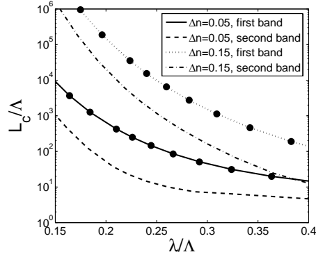
Fig. 5. Coupling length for different index contrasts for a structure with d/\Lambda = 0.5 . The refractive index of the background is fixed at 1.44, corresponding to silica at \lambda_0 = 1.5\mu\text{m} . The black dots show the result of the coupled mode approximation for the first band.
